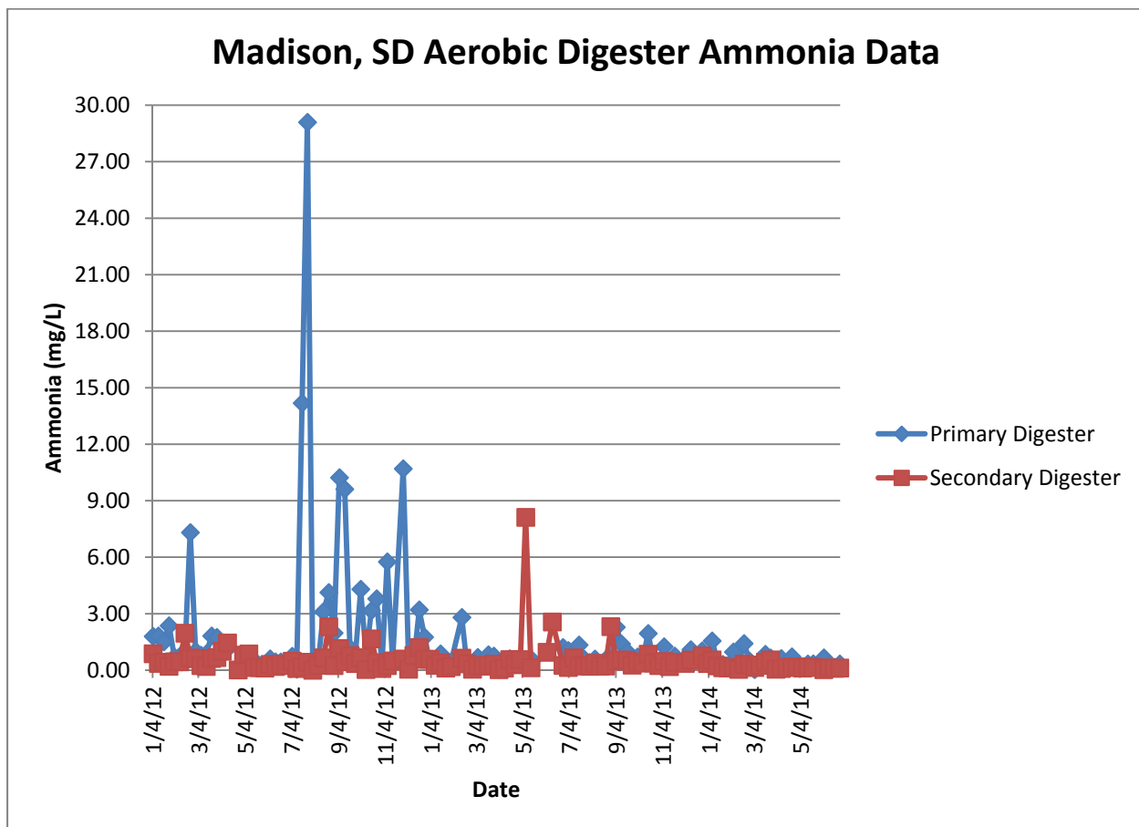
Figure 6: Madison, SD WWTP Aerobic Digestion System Ammonia Data
