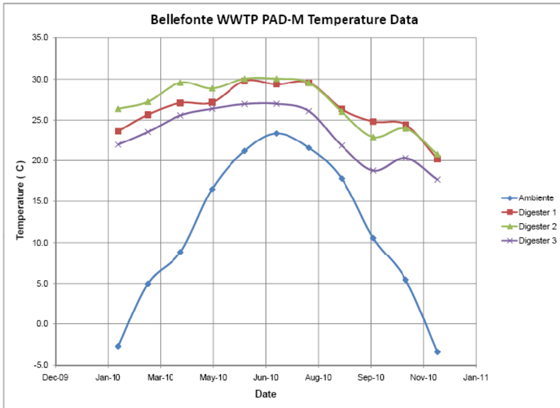
Figure 2. Bellefonte WWTP P.A.D.-M Process Temperature Data
