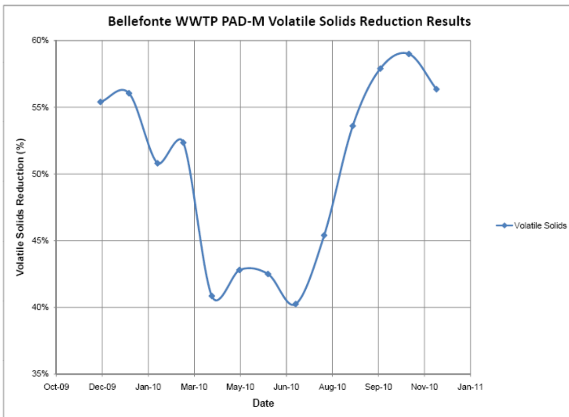
Figure 3. Bellefonte WWTP Volatile Solids Reduction Performance
